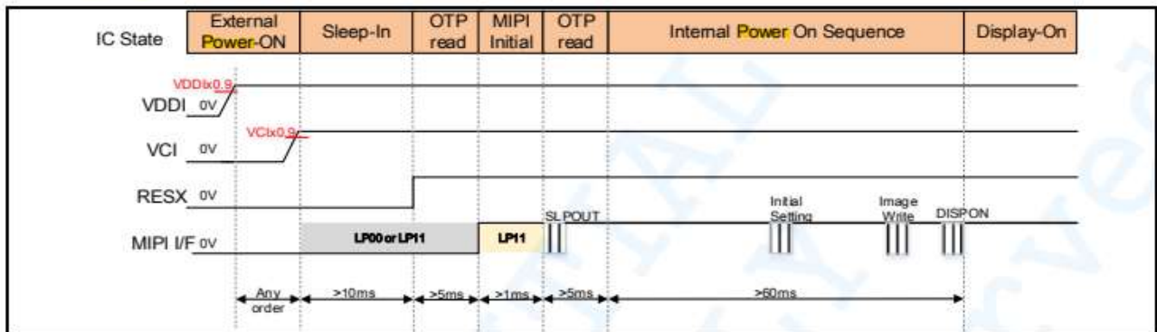
Figure 15 Power-On Sequence
