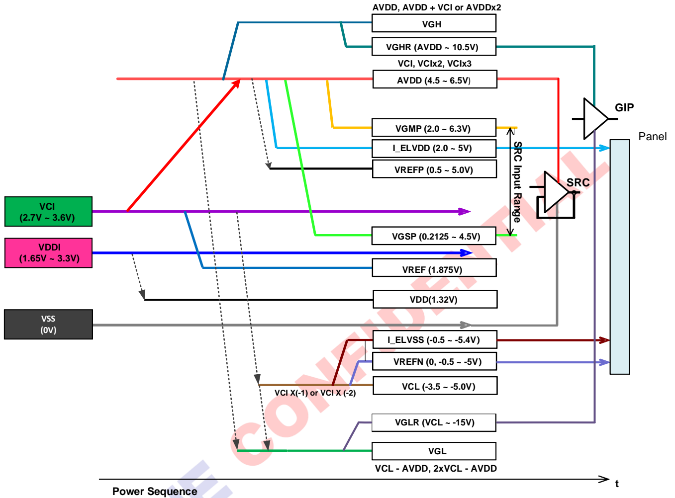
Power Stage Diagram
