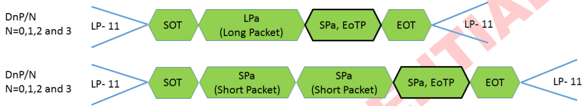
End of Transmission Packet (EoTP) – Example
