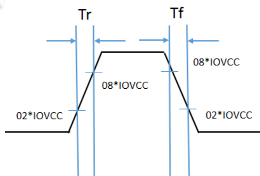
Figure 6-16 Tearing effect output line – definition of Tr,Tf
