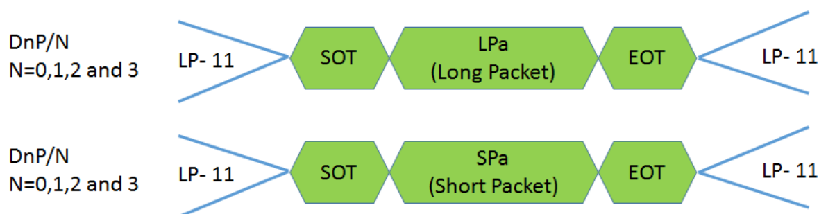
Figure 5-18 Single Packet in High- Speed Data Transmissions
