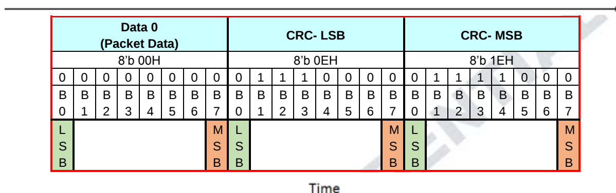
Figure 5-43 Packet Footer (PF) Example
