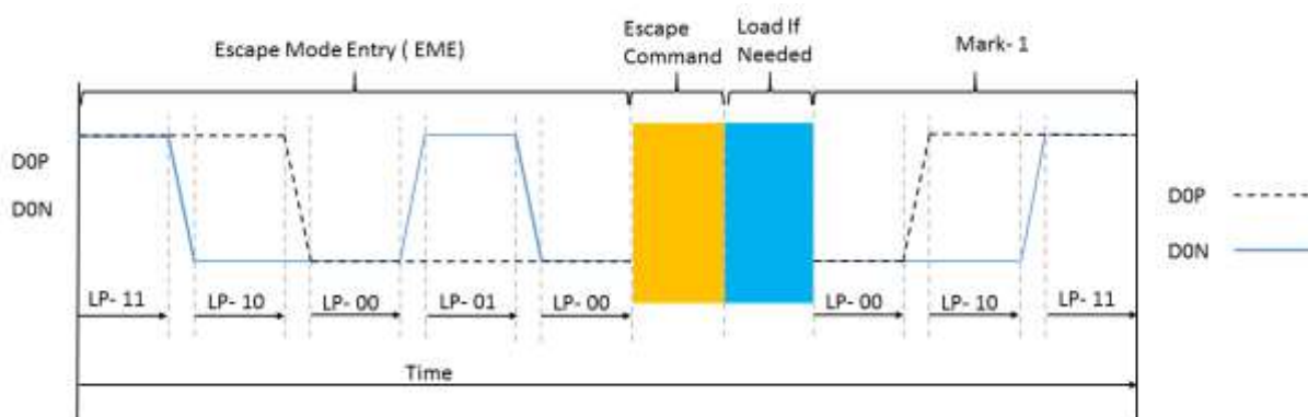
Figure 5-10 General Escape Mode Sequence
