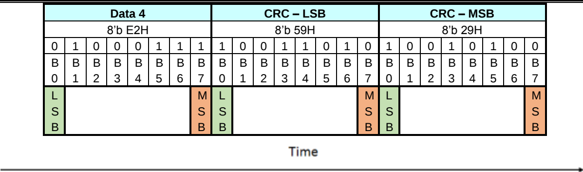
Figure 5-52 Null Packet, No Data (NP- L) – Example
