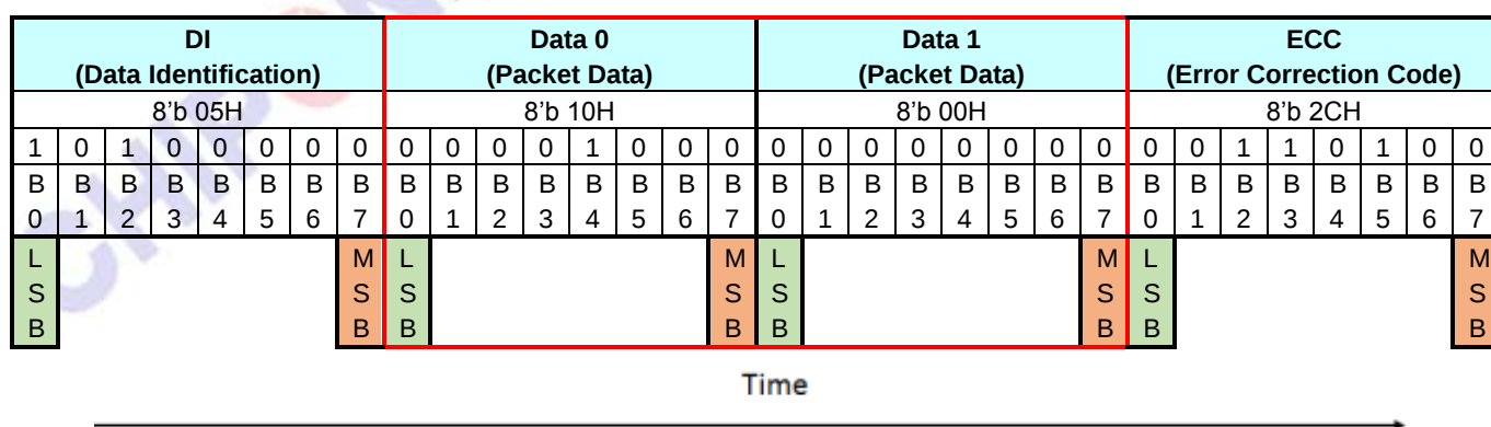
Figure 5-33 Packet Data (PD) for Short Packet (SPa), 1 Byte Information
