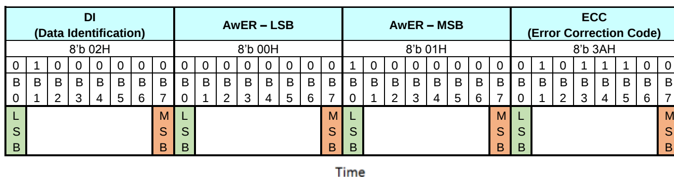
Figure 5-55 Acknowledge with Error Report (AwER) – Example
