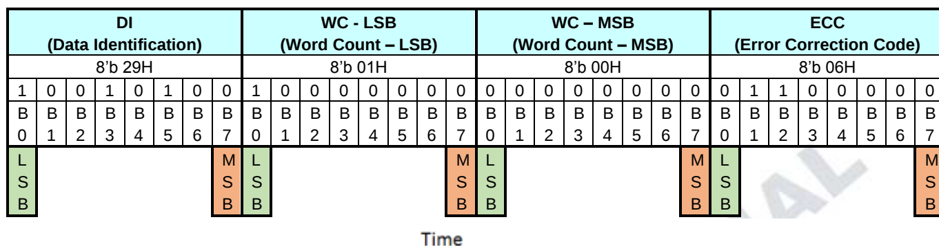
Figure 5-23 Bit order of the byte on packet
