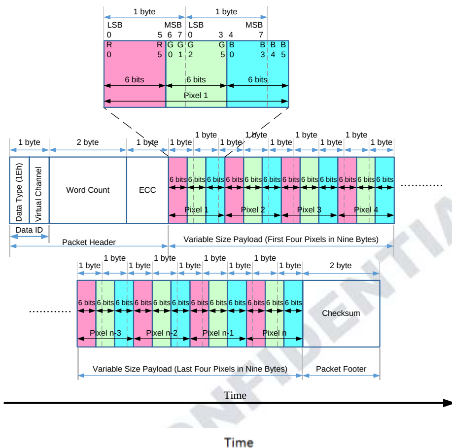
Figure 5-65 18-bit per Pixel – RGB Color Format, Long Packet
