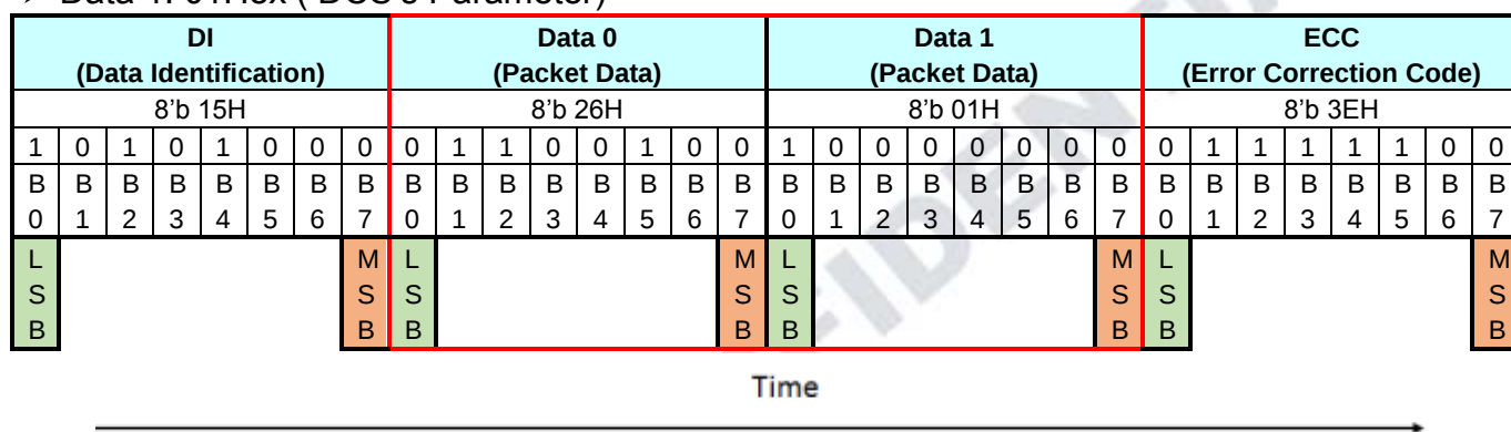
Figure 5-32 Packet Data (PD) for Short Packet (SPa), 2 Bytes Information
