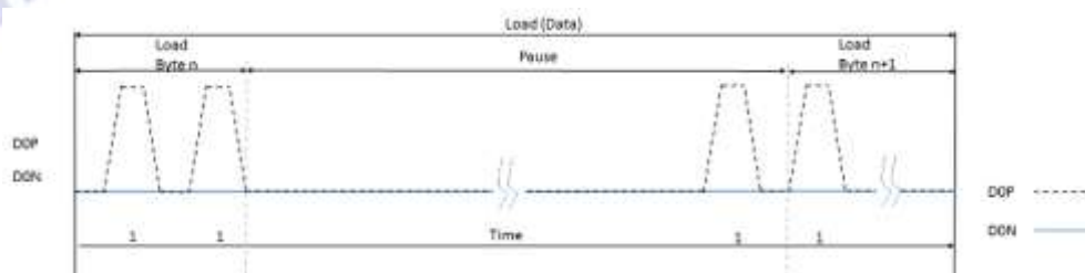
Figure 5-12 Pause (Example)
