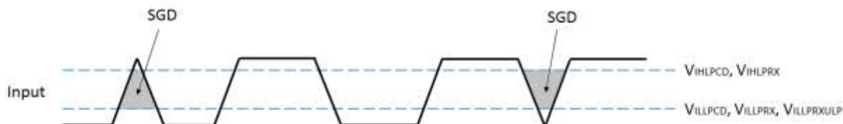
Figure 4-1 Spike/Glitch Rejection
