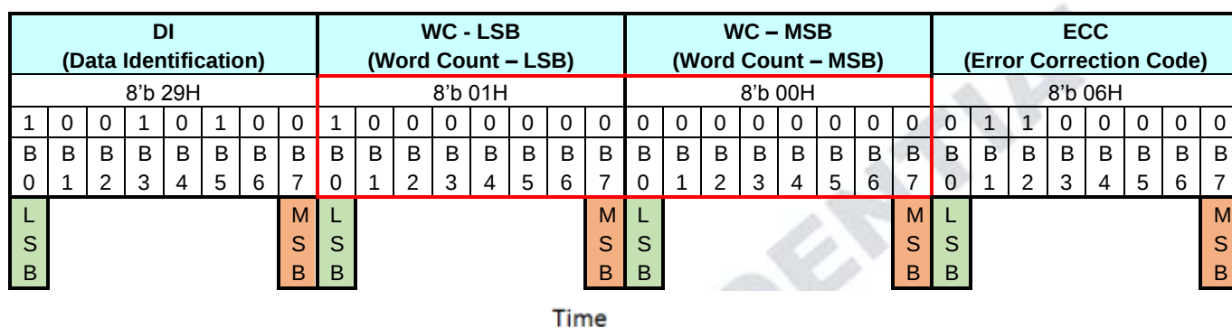
Figure 5-34 Word Count (WC) in a Long Packet (LPa)
