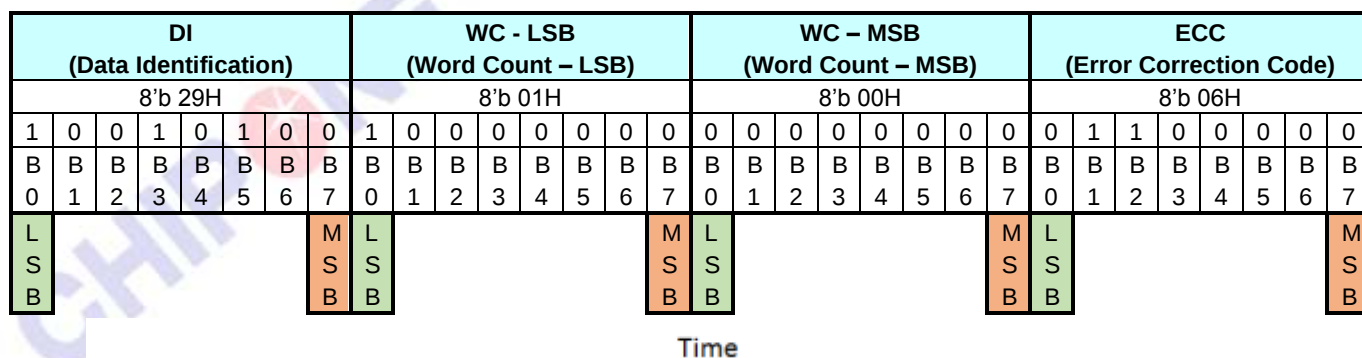
Figure 5-26 Packet Header (PH) in a Long Packet (LPa)
