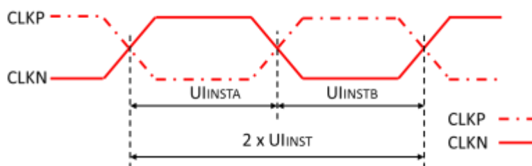
Figure 4-5 Clock Timing
