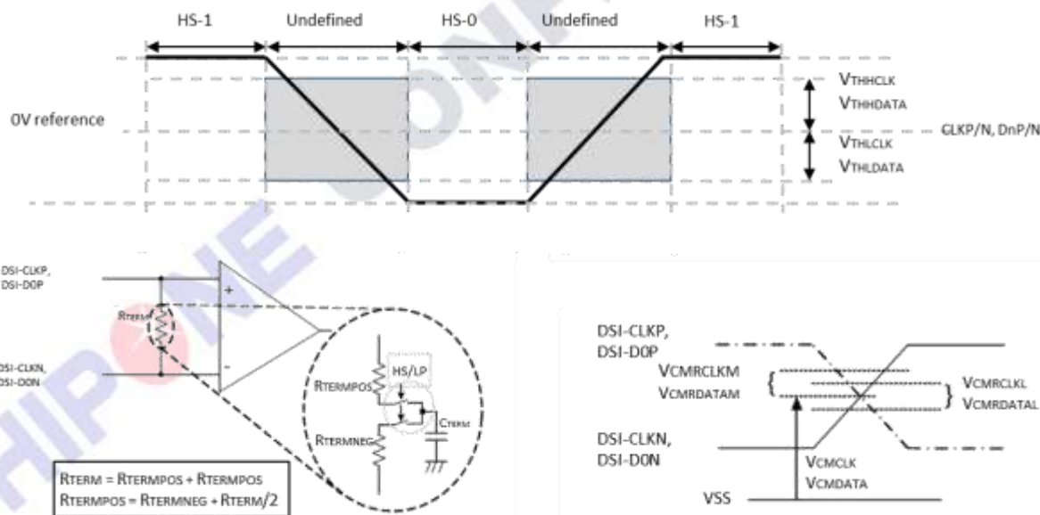
Figure 4-2 Differential voltage range, termination resistor and Common mode voltage
