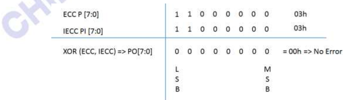
Figure 5-39 Internal XOR Calculation between ECC and IECC Values – No Error
