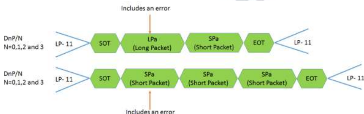
Figure 5-56 Error Packets
