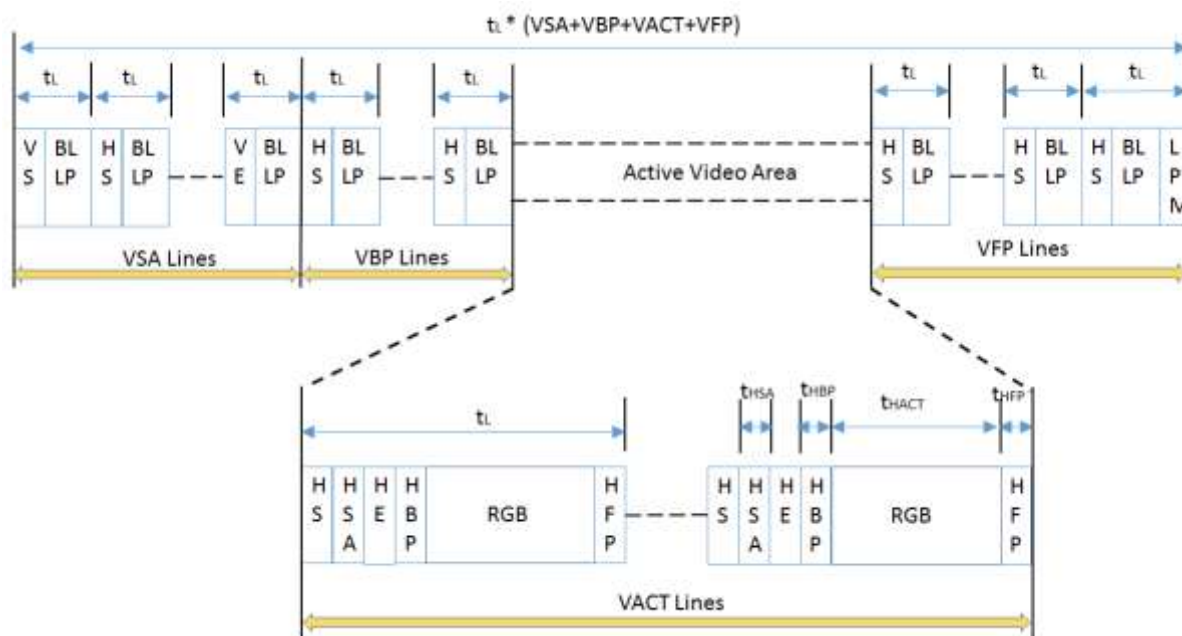
Figure 5-62 DSI Video Mode Interface Timing: Non-Burst Transmission with Sync Start and End
