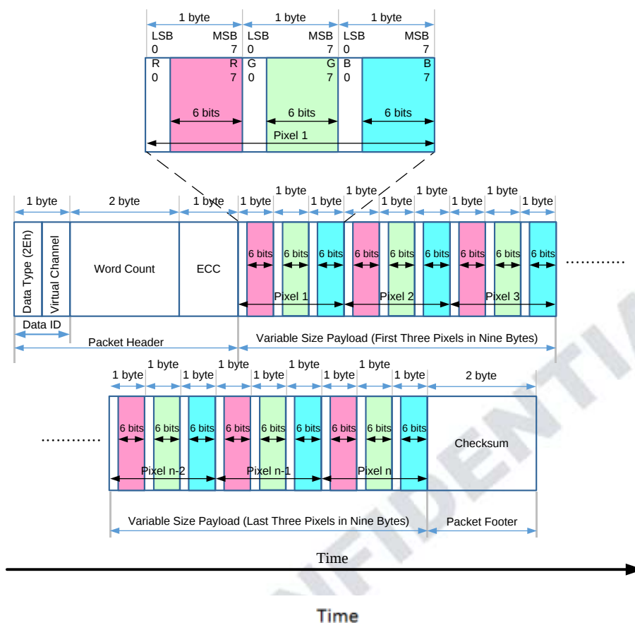
Figure 5-66 18-bit per Pixel (Loosely Packed) – RGB Color Format, Long Packet
