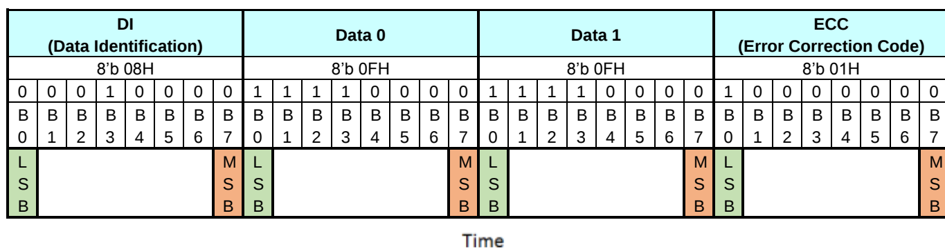
Figure 5-53 End of Transmission Packet (EoTP)
