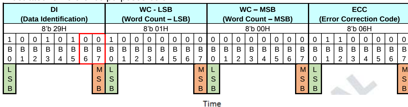
Figure 5-29 Virtual Channel (VC) on the Packet Header (PH)
