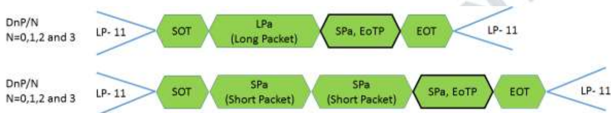
Figure 5-54 End of Transmission Packet (EoTP) – Example
