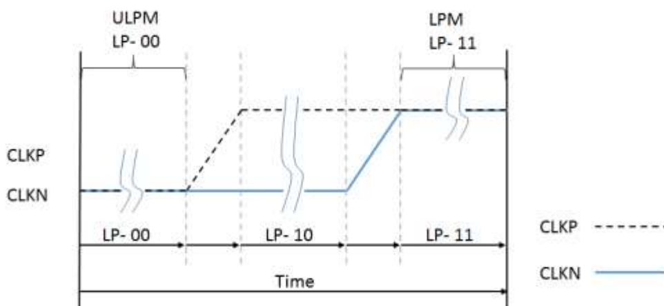
Figure 5-2 From ULPM to LPM
