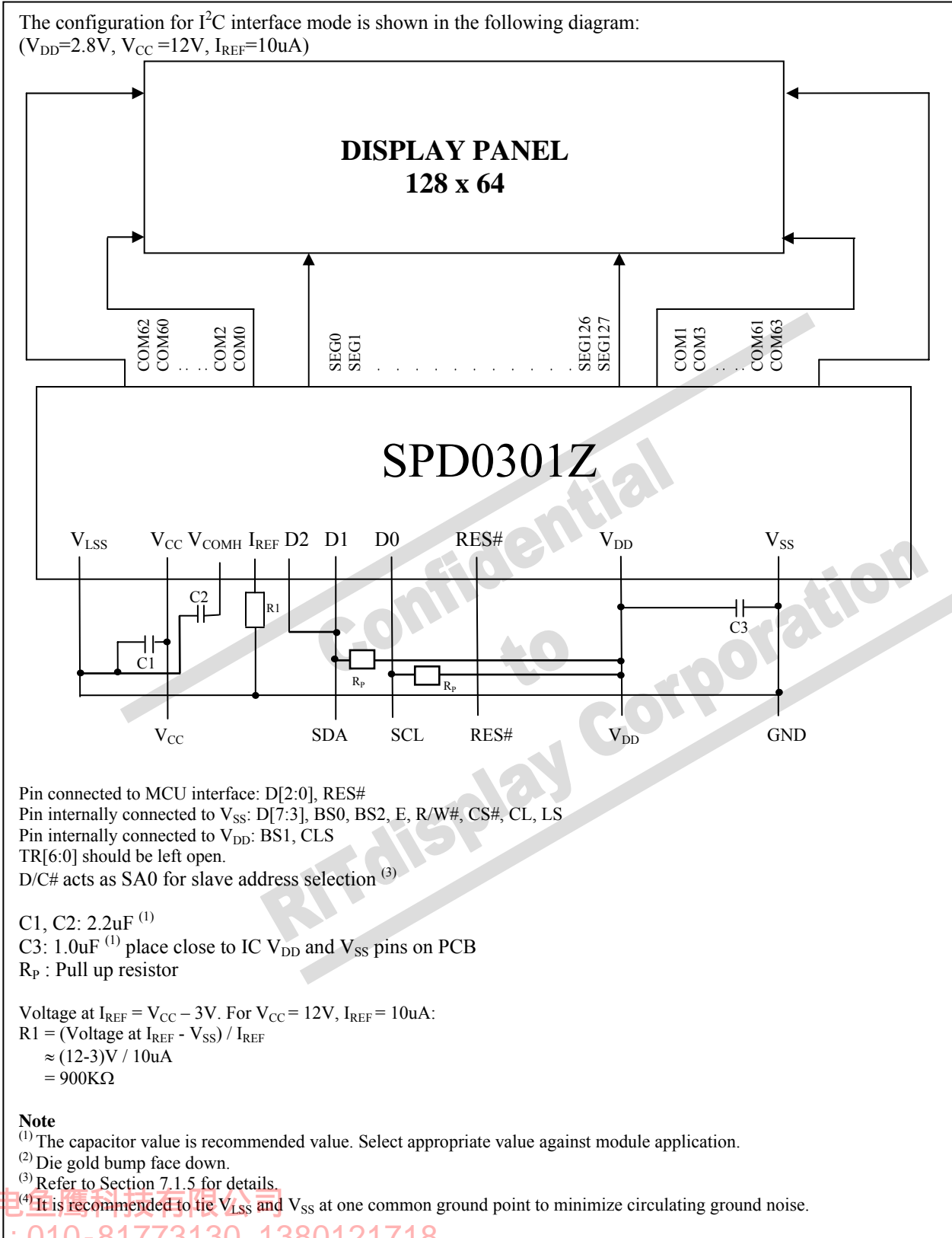
Figure 13-1 : Application Example of SPD0301Z
